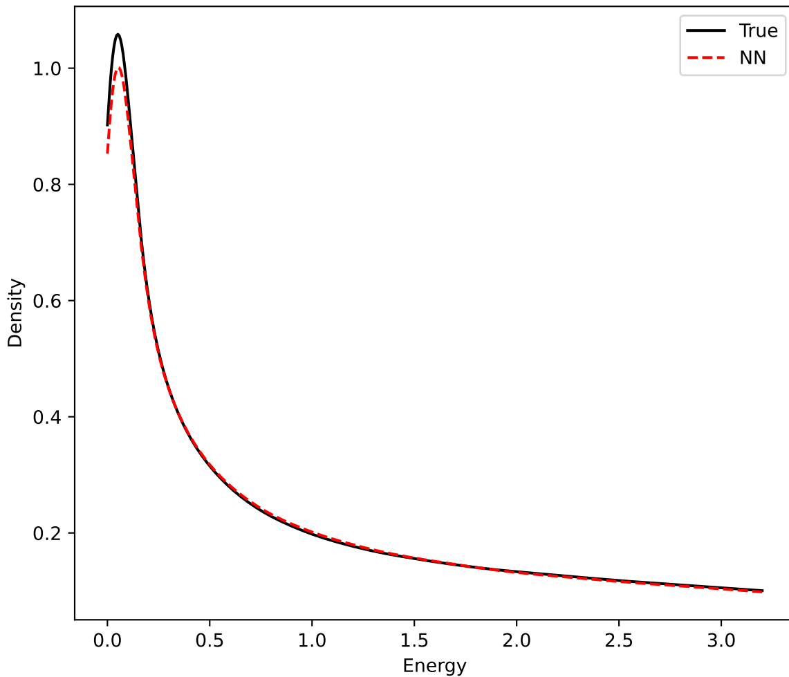
TKE Density Comparison with KS: 0.0097, p-value: 0
